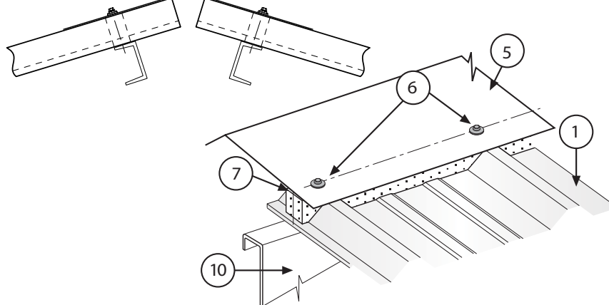
Typical Ridge Trim Detail Figure 26d
