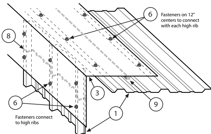
Typical Gable Trim Detail Figure 26b
