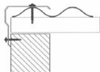
Cross section: Styled Gable Trim - 90° Figure 19b
