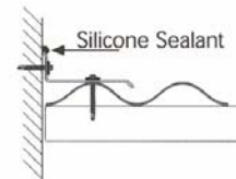
Cross section: Side Wall Trim - 90° Figure 21b
